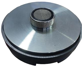
TW156 40.000 Driver 60w, bobina 34,4mm, peso 970gr
