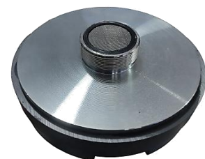
TW158 80.000 Driver 120w, bobina 51,6mm, peso 2830gr
